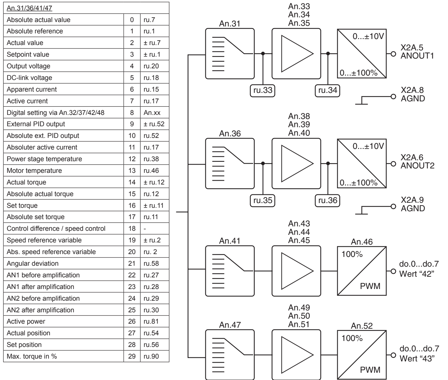
Figure 7.2.9 Principle of the analog inputs
