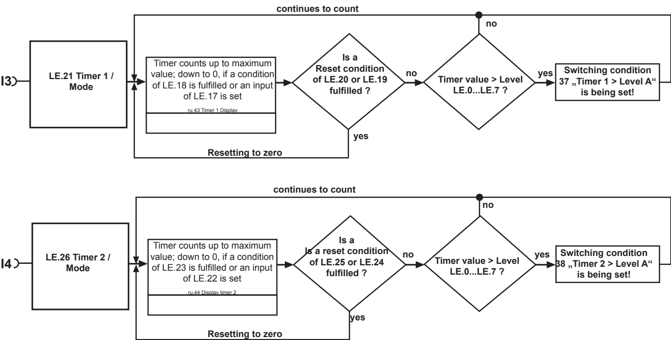
Fig. 7.15.4 Timer programming
