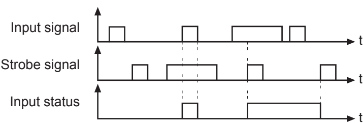
Figure 7.3.8.b Static strobe mode 1 (di.07 = 1)
